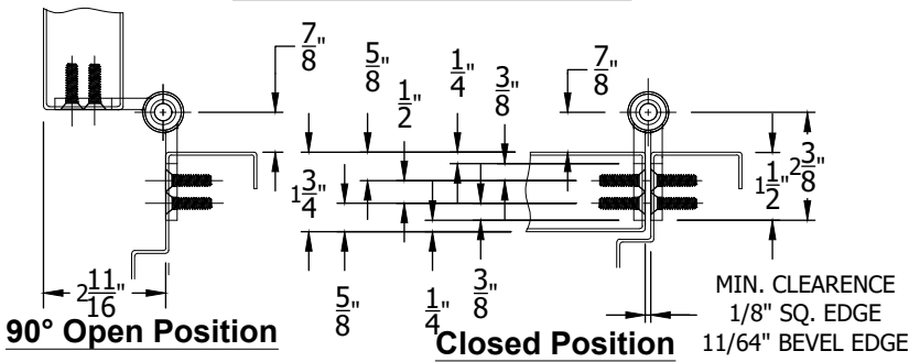
RIGHT HANDED HINGE SHOWN
