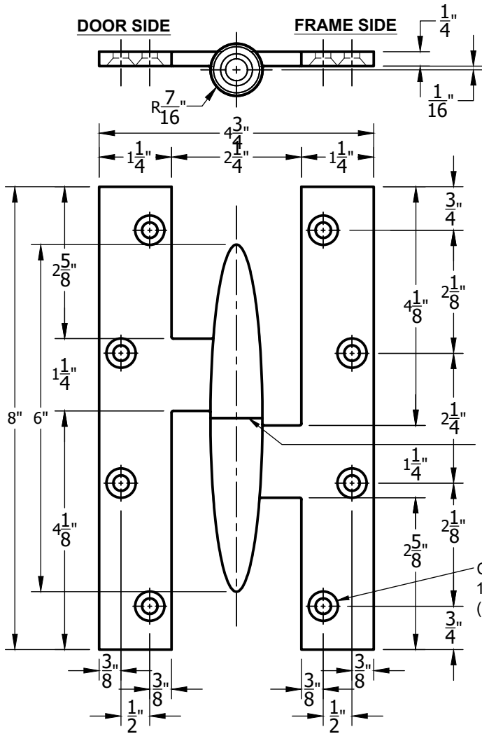
RIGHT HANDED HINGE SHOWN
