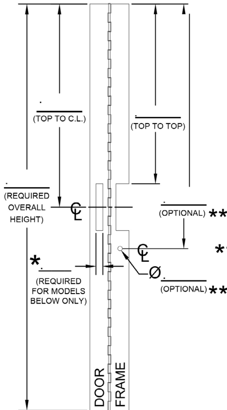
STAINLESS STEEL PIN & BARREL HINGE
