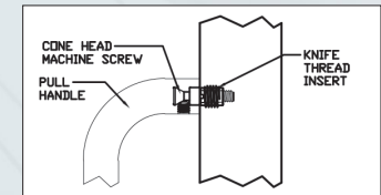
Glass Door Back-to-Back Type 13HD
