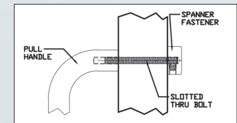
Thru Bolt - Type 12HD
