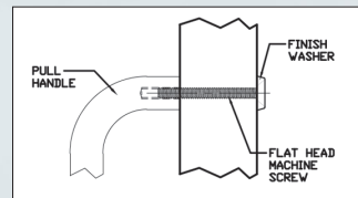
Thru Bolt - Type 1HD
