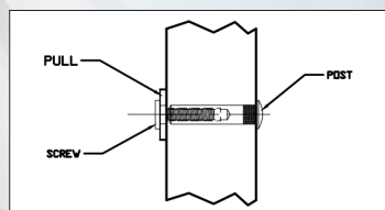
Thru Bolt
