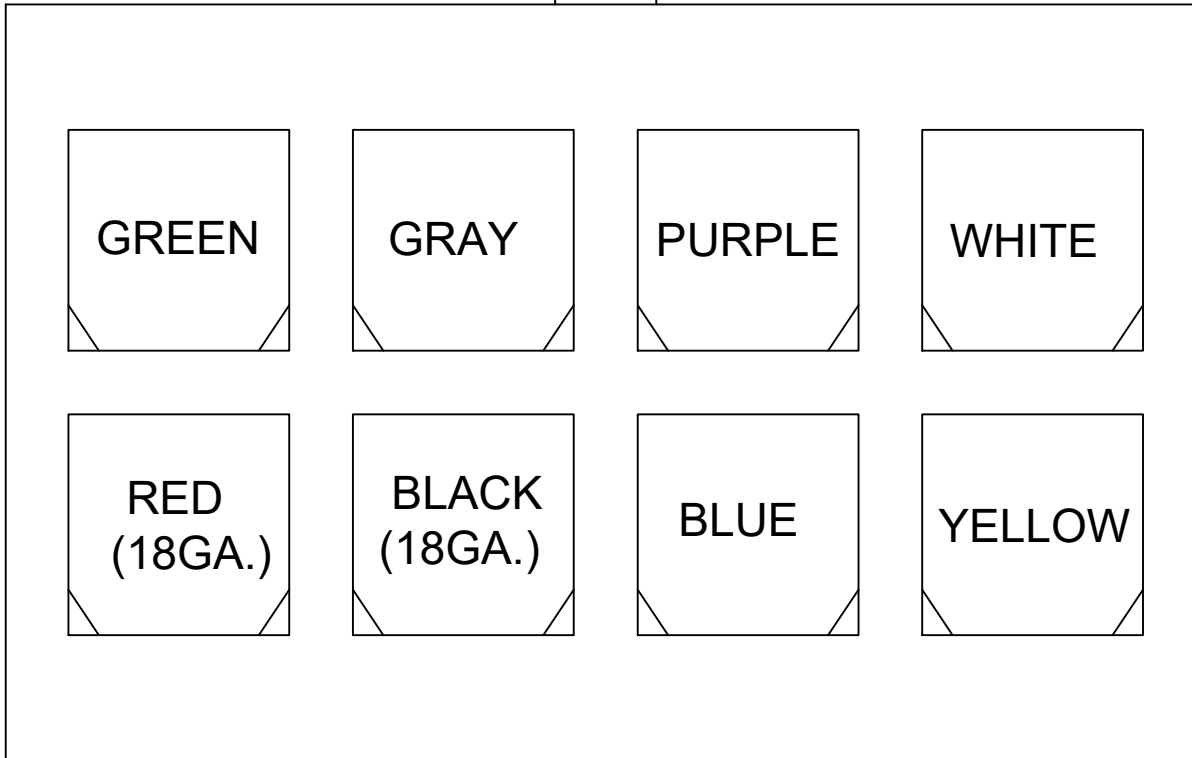
8 - MALE PIN HOUSING MOLEX CONNECTOR MICRO-FIT 3.0 (43020-0801) ABH-3303
