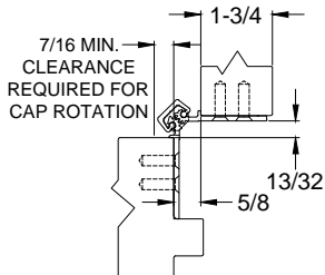
90° OPENING
