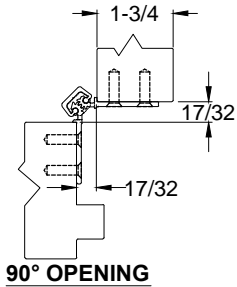
90° OPENING
