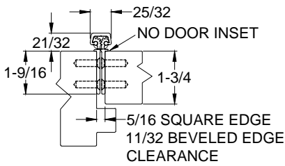
CLOSED POSITION
