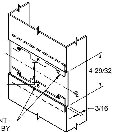
CUT-OUT FOR METAL JAMB
