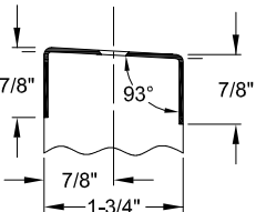
A528BO ● BEVELED EDGE ● OVERLAPPING
