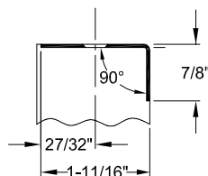
A528SM ● SQUARE EDGED ● MORTISED
