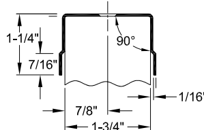
A538SO ● SQUARE EDGED ● OVERLAPPING BOTH SIDES ● NON-MORTISED
