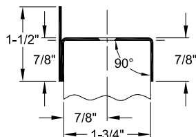
A548S ● SQUARE EDGED ● NON-MORTISED
