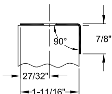
A528S ● SQUARE EDGED ● NON-MORTISED
