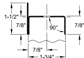
A548SM ● SQUARE EDGED ● MORTISED
