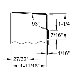
A528BO ● BEVELED EDGE ● OVERLAPPING
