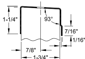
A538BO-1 ● BEVELED EDGE ● OVERLAPPING ONE SIDE ● NON-MORTISED
