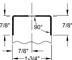
A528SO ● SQUARE EDGED ● OVERLAPPING
