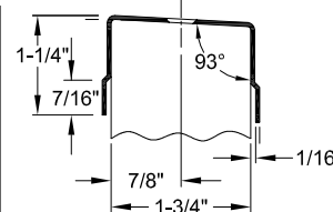
A538BO ● BEVELED EDGE ● OVERLAPPING BOTH SIDES ● NON-MORTISED
