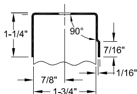
A538SO-1 ● SQUARE EDGED ● OVERLAPPING ONE SIDE ● NON-MORTISED
