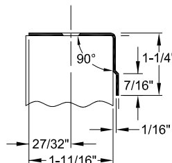
A528SO ● SQUARE EDGED ● OVERLAPPING
