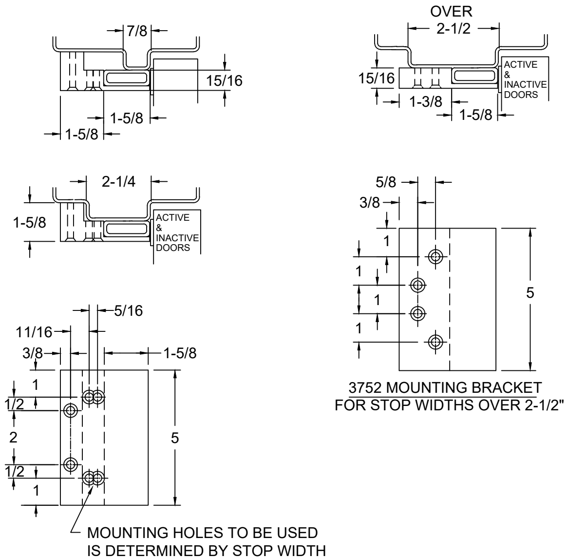
3751 MOUNTING BRACKET FOR STOP WIDTHS UP TO 2-1/2"
