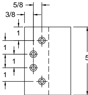
3752 MOUNTING BRACKET FOR STOP WIDTHS OVER 2-1/2"
