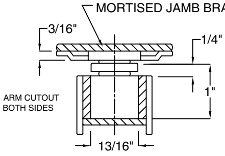
DOUBLE ACTING DOOR
