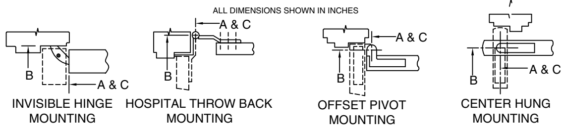
DOUBLE ACTING DOOR
