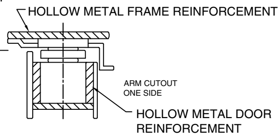
SINGLE ACTING DOOR
