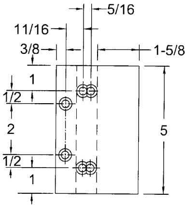
3751 MOUNTING BRACKET FOR STOP WIDTHS UP TO 2-1/2"
