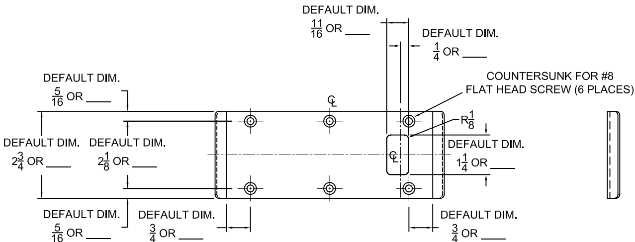
FRONT VIEW
